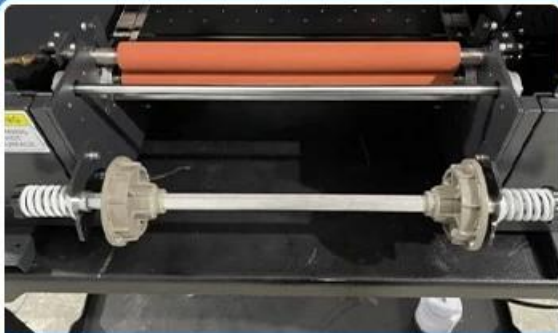
Printing and laminating 2 in 1 for efficient production.
